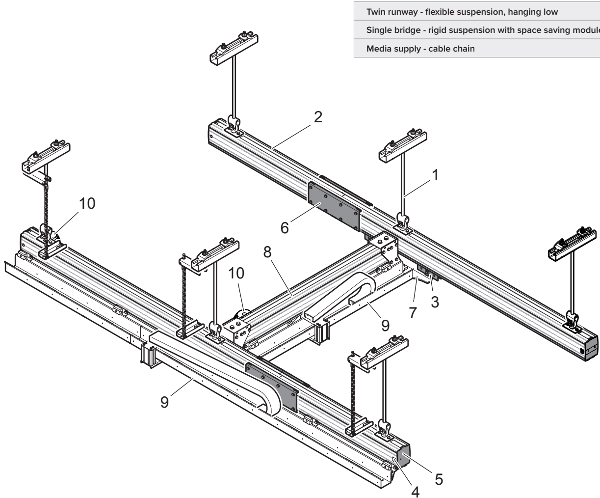
Example 4: Single bridge with space saving module
