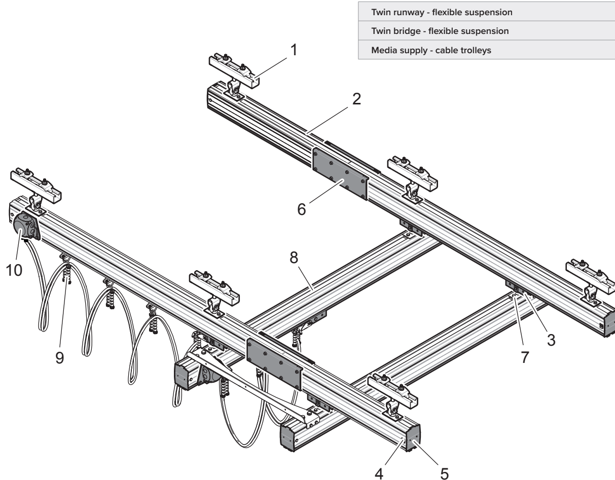
Example 5: Twin bridge
