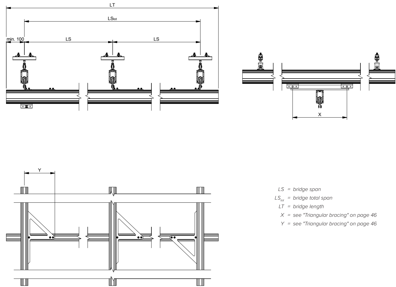
Triple track system
