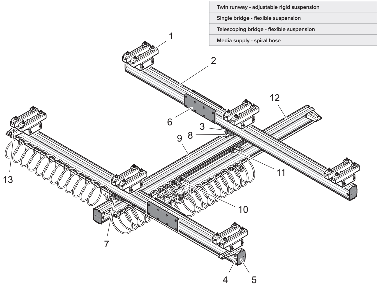
Example 11: Telescoping single bridge
