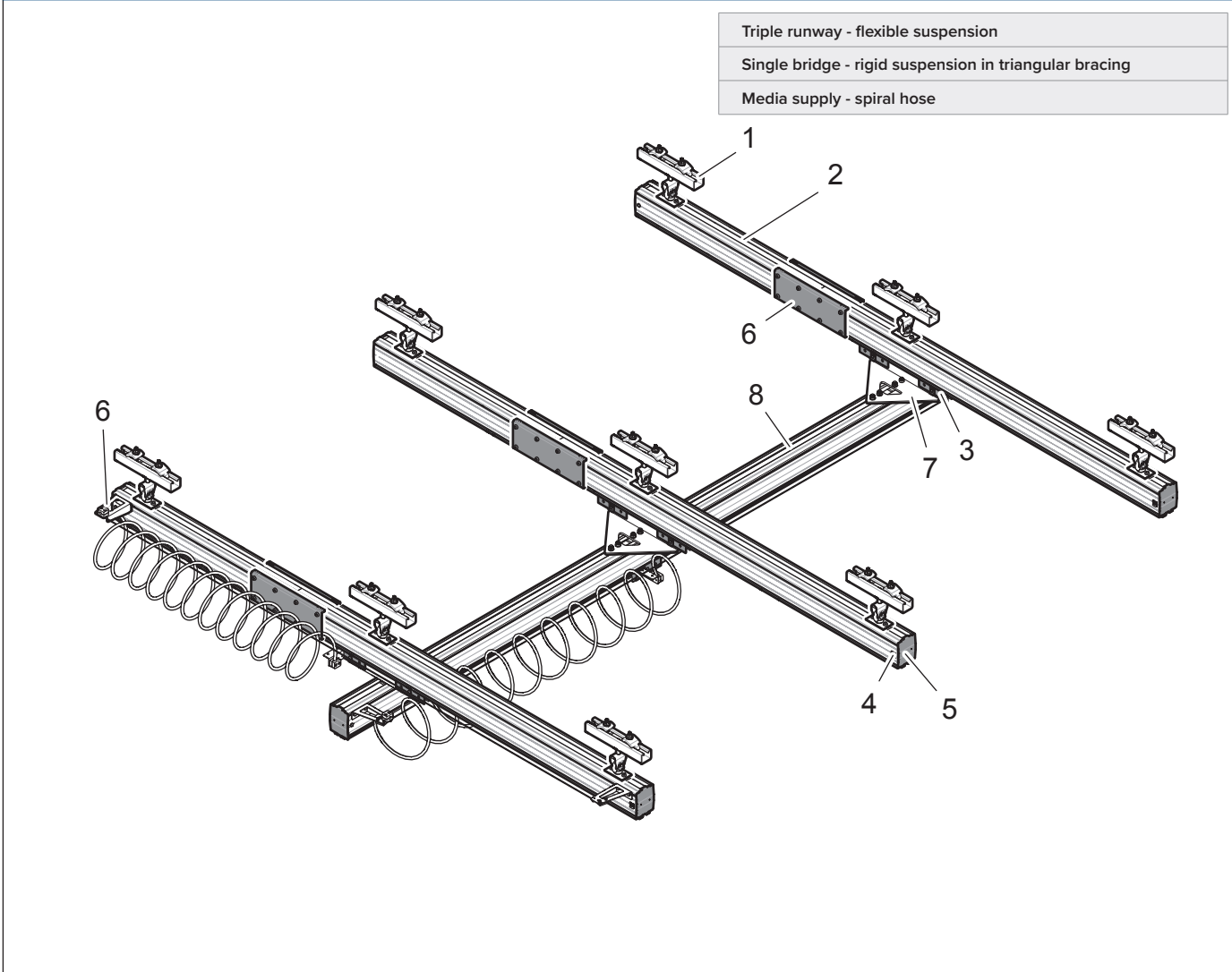
Example 7: Triple runway
